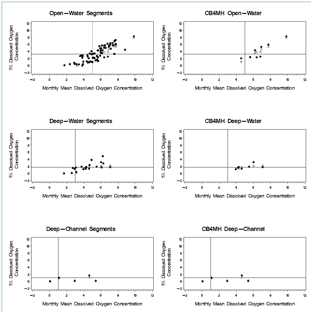
Figure V-1. Plots of monthly mean dissolved oxygen concentration ( \text{mg liter}^{-1} ) versus the 1 percentile dissolved oxygen concentration as measured by sensors on individual buoys. Plots on left side show patterns of dissolved oxygen concentration data pooled across Chesapeake Bay Program segments within open-water, deep-water and deep-channel uses. Plots on the right side show patterns of dissolved oxygen concentration data from middle central Chesapeake Bay, segment CB4MH. Circles are observed dissolved oxygen concentration data; open triangles are dissolved oxygen concentrations predicted by the regression model: 1 percent dissolved oxygen concentration as a function of monthly mean dissolved oxygen and the coefficient of variation.
