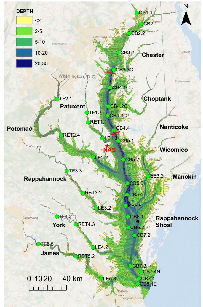
FIGURE 1. Chesapeake Bay, simulation grid, bathymetry (m), tributaries, and observation stations for model calibration. The red star is the Naval Air Station (NAS) from which surface forcing data were collected. Red lines are the boundary of the central segment CB4MH spanning from the mouth of the Chester River to the north to the mouth of the Patuxent River to the south.
