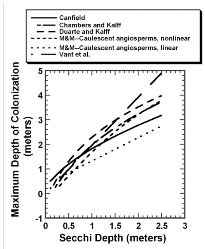
FIGURE III-1. Modeled Relationships of Maximum Depth of Colonization to Secchi Depth for Freshwater Lake SAV Species. Relationship of maximum depth of colonization ( Z_{\text{max}} ) to Secchi depth for freshwater SAV species as modeled by Canfield et al. (1985), Chambers and Kalff (1985), Duarte and Kalff (1987), Middleboe and Markager (1997) and Vant et al. (1986).
