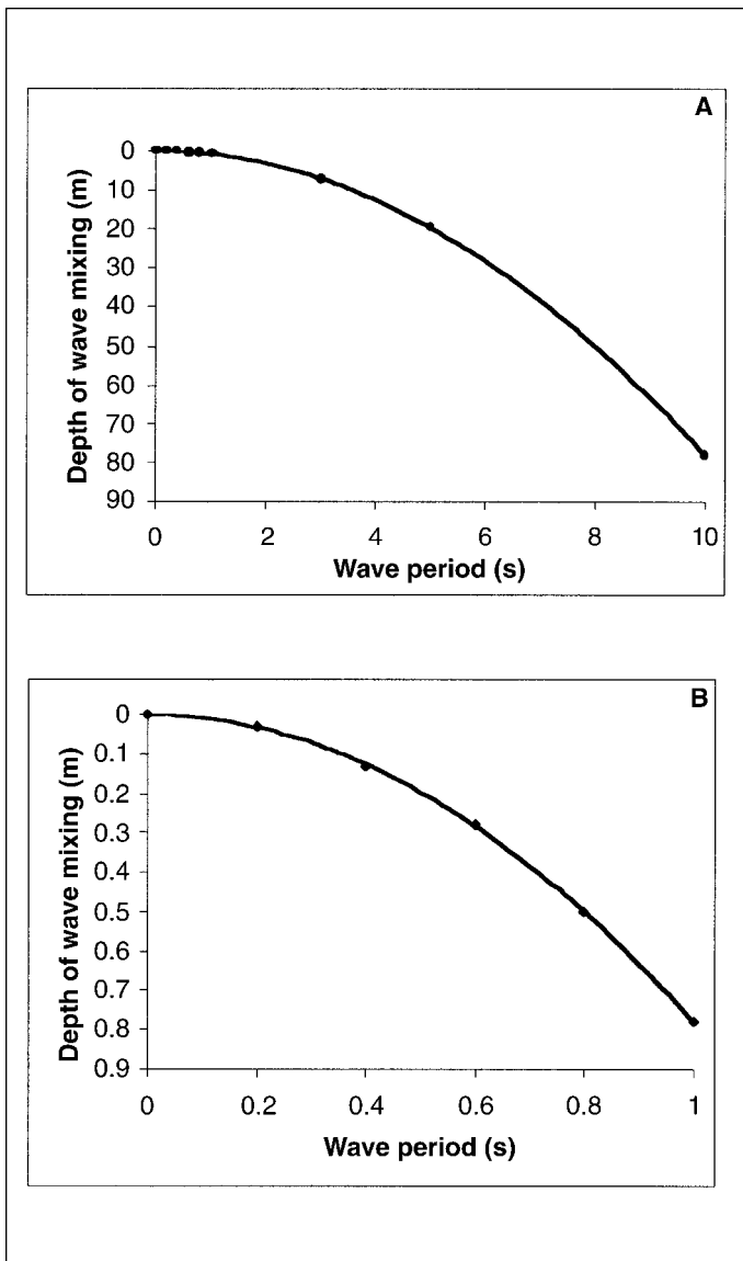
FIGURE VI-3. Wave Period/Depth of Wave Mixing Relationship. Depth of wave mixing (or minimum depth of distribution of SAV) under a variety of wave conditions. Wind-generated waves are typical for relatively exposed areas (A) while ripples are typical for shallow coastal areas. SAV occur in habitats characterized by both wave types. Depth of wave mixing for waves periods more characteristic of SAV habitats in Chesapeake Bay are illustrated in B.
