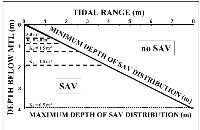
FIGURE VI-6. Effect of Increased Light Attenuation on Maximum Depth of SAV Distribution. The magnitude of the effect of increased light attenuation ( K_d ) on the maximum depth of SAV distribution as determined based on the equations presented in the text, assuming a SAV minimum light requirement of 13 percent. MTL is the mean tide level.
