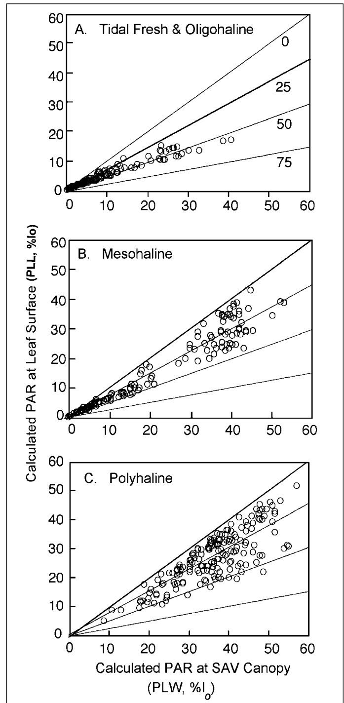
FIGURE 3. Percent Light at Leaf vs. Percent Light Through Water Column by Salinity Regime. Comparing values for percent surface light at SAV leaf surface (PLL) and percent surface light through water just above the SAV leaf (PLW) calculated for Z = 1 m from the model described in this report (Table V-1) for water quality monitoring stations in Virginia portion of Chesapeake Bay for 1985-1996 in three salinity regimes. Lines indicate position of points where epiphyte attenuation reduced ambient light levels at the leaf surface by 0, 25, 50 and 75 percent.
