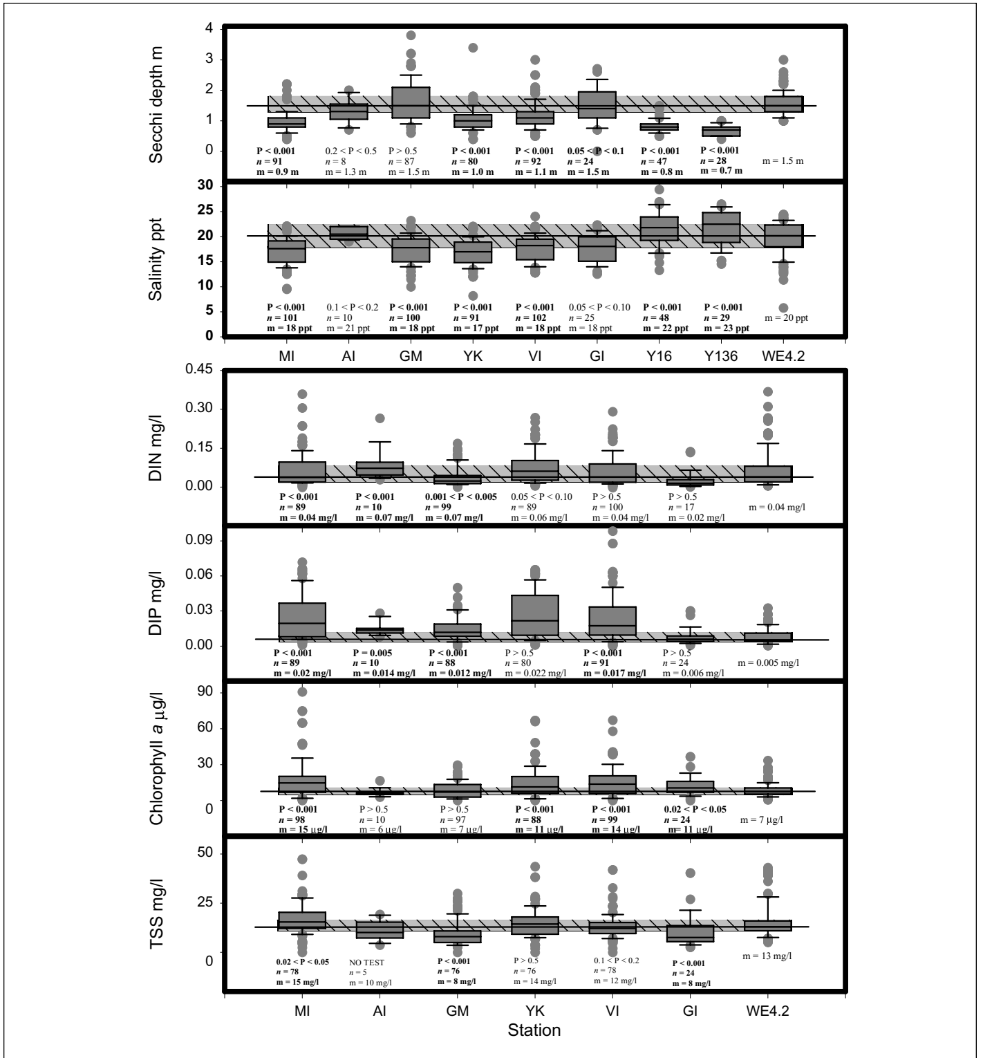
FIGURE IX-2. Representative box plot (from Lower York River). Circles above and below each plot are outliers. Grey band with diagonal black lines shows the interquartile range of the midchannel data. The solid line extending horizontally through all plots shows the median of the midchannel data. Under each plot are the results of the Wilcoxon rank-pair test, the n of the test and the median from each station’s data. Stations MI, AI, GM, YK and GI are Virginia Institute of Marine Science stations, Y16 and Y136 are citizen monitoring stations managed by the Alliance for the Chesapeake Bay.
