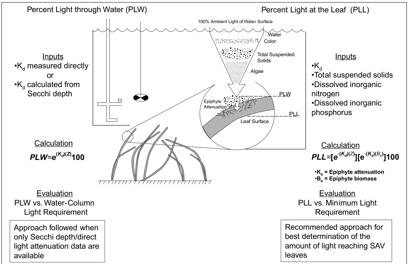
FIGURE VII-2. Calculation of PLW and PLL and Comparisons with their Respective Light Requirements. Illustration of the inputs, calculation, and evaluation of the two percent light parameters: percent light through water and percent light at the leaf.
