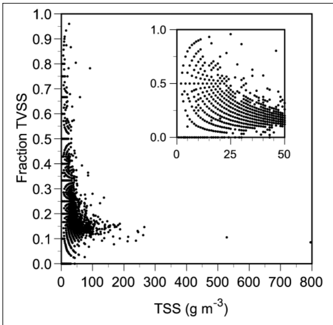
FIGURE IV-3. Fraction of Total Suspended Solids Lost on Ignition. Fraction of total suspended solids (TSS) that is lost on ignition as a function of TSS. At concentrations of TSS < 50 \text{ mg liter}^{-1} (inset), the fraction of TSS that is volatile varies from 0 to >90 percent. Total volatile suspended solids (TVSS) calculated as total suspended solids minus fixed suspended solids, that is, the mass remaining after combustion. Fraction total volatile suspended solids calculated as total volatile suspended solids divided by total suspended solids. Data from Chesapeake Bay Water Quality Monitoring Program, Virginia tidal tributary stations, 1994-1996.
