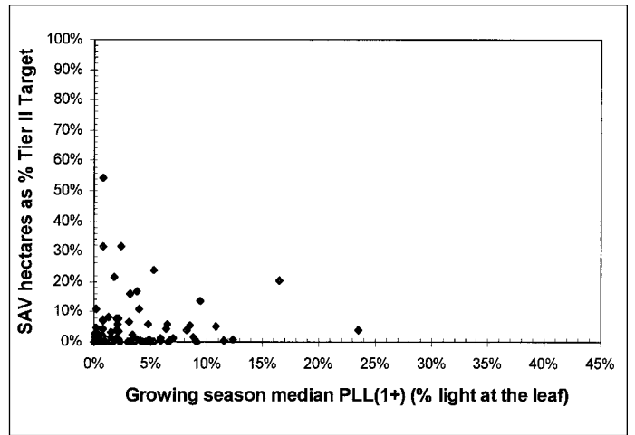
FIGURE VII-6. Oligohaline SAV Area vs. Percent Light at the Leaf. Oligohaline SAV area as a percent of the Tier II SAV distribution restoration target by year and Chesapeake Bay Program segment vs. median percent light at the leaf [PLL(1+)] by year and Chesapeake Bay Program segment, using 1985-1998 data (no data from 1988). Spearman r_s = 0.37 , N = 182 , P = 0.0001 .
