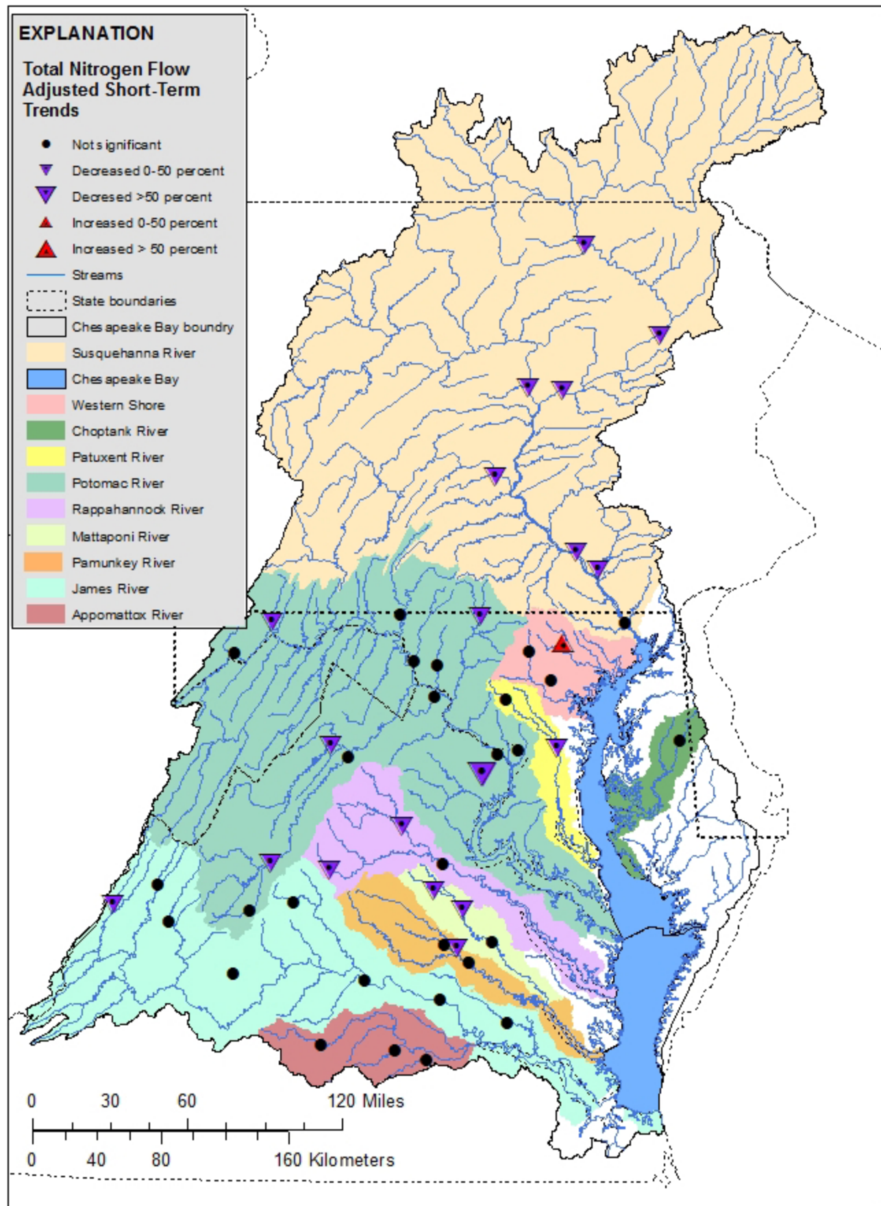
Flow-adjusted trends for total nitrogen for 48 sites in the Chesapeake Bay Watershed, 2002-2011.
