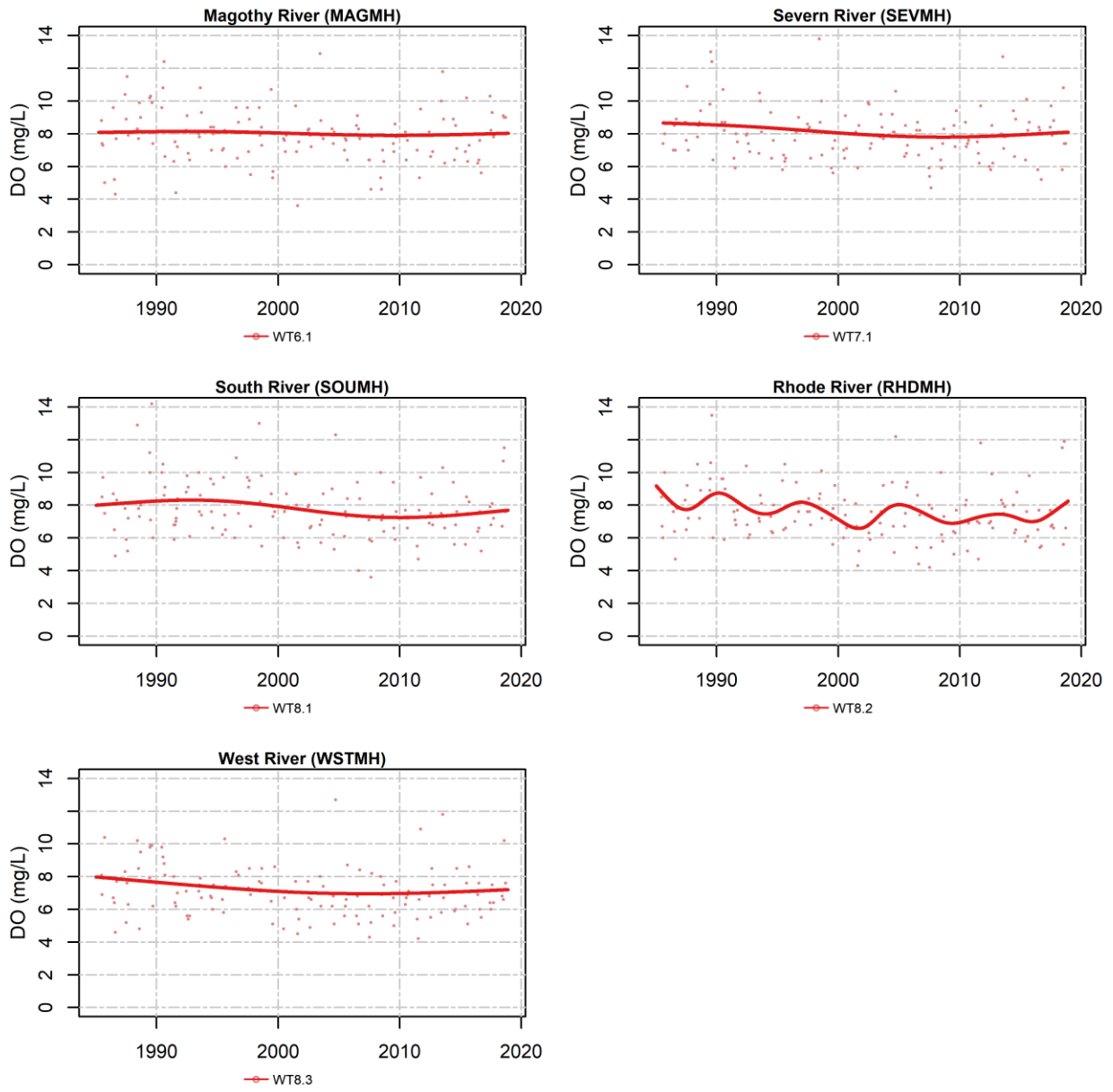
Figure A-12. Summer (June-Sept) surface DO data (dots) and summer mean long-term pattern generated from non-flow adjusted GAMs.
