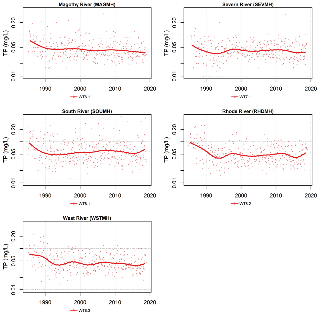
Figure A-4. Bottom total phosphorus data (dots) and average long-term pattern generated from non-flow adjusted GAMs.
