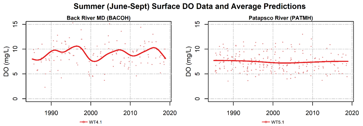
Figure A-12. Summer (June-Sept) surface DO data (dots) and summer mean long-term pattern generated from non-flow adjusted GAMs.
