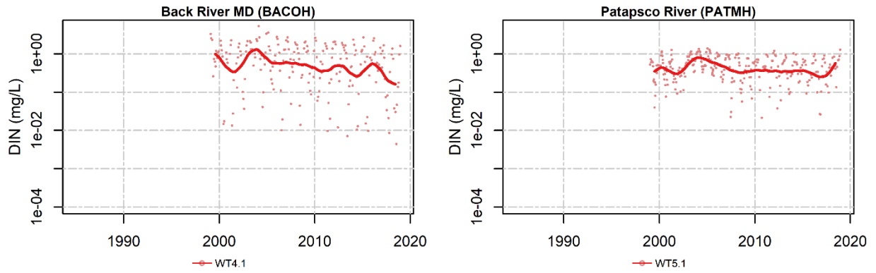
Figure A-6. Surface DIN data (dots) and average long-term pattern generated from non-flow adjusted GAMS.
