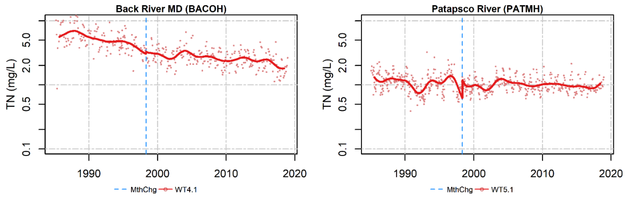
Figure A-2. Bottom total nitrogen data (dots) and average long-term pattern generated from non-flow adjusted GAMs.
