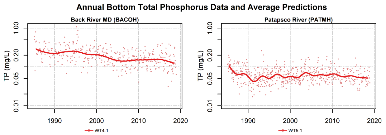
Figure A-4. Bottom total phosphorus data (dots) and average long-term pattern generated from non-flow adjusted GAMs.
