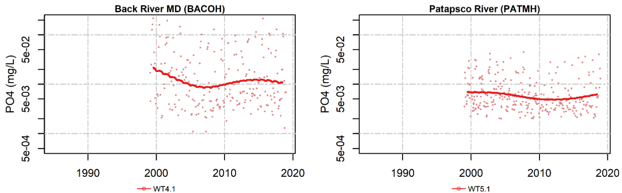
Figure A-8. Surface orthophosphate data (dots) and average long-term pattern generated from non-flow adjusted GAMs.
