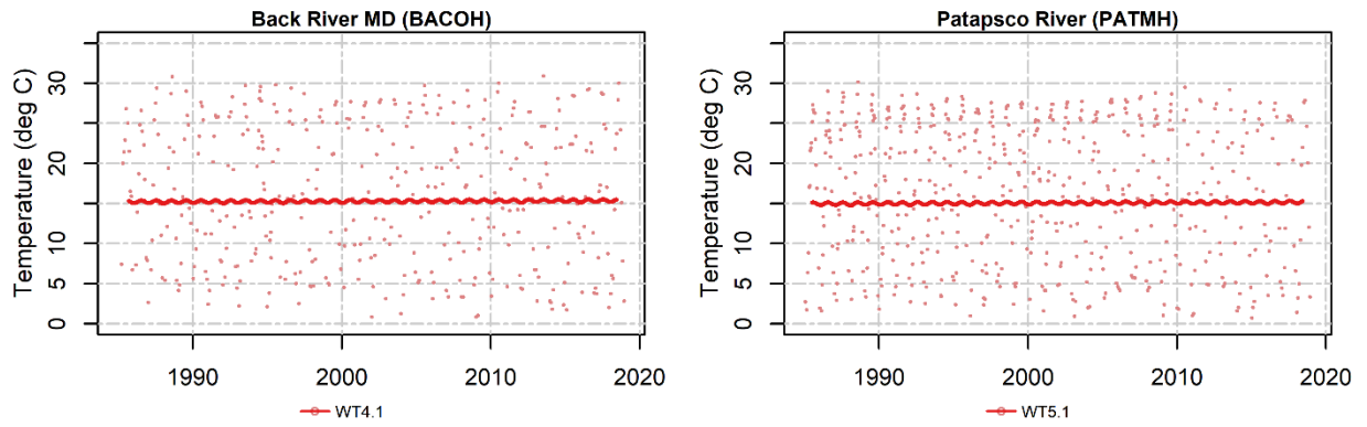
Figure A-14. Surface water temperature data (dots) and average long-term pattern generated from non-flow adjusted GAMs.
