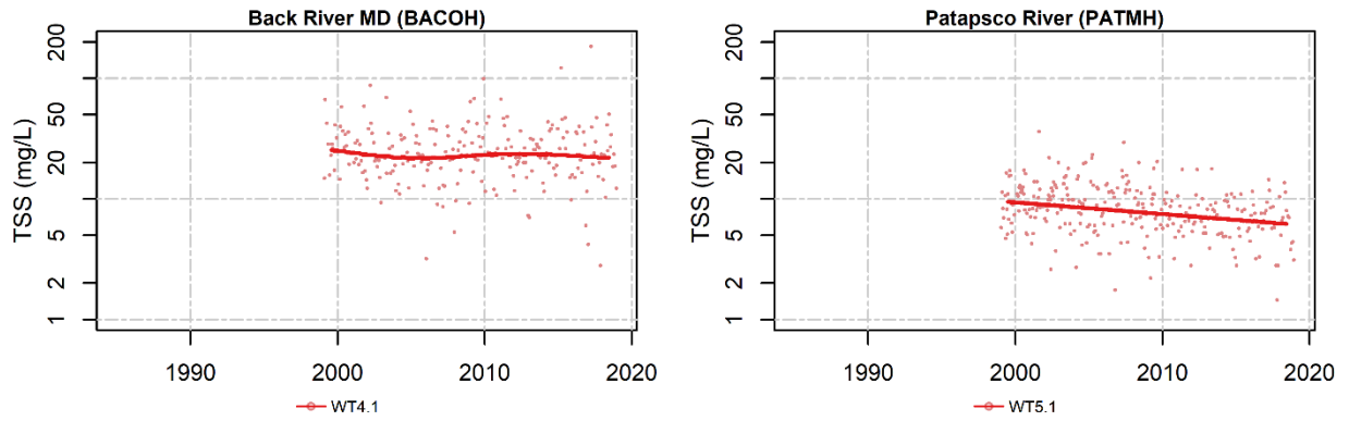
Figure A-10. Surface TSS data (dots) and average long-term pattern generated from non-flow adjusted GAMS.
