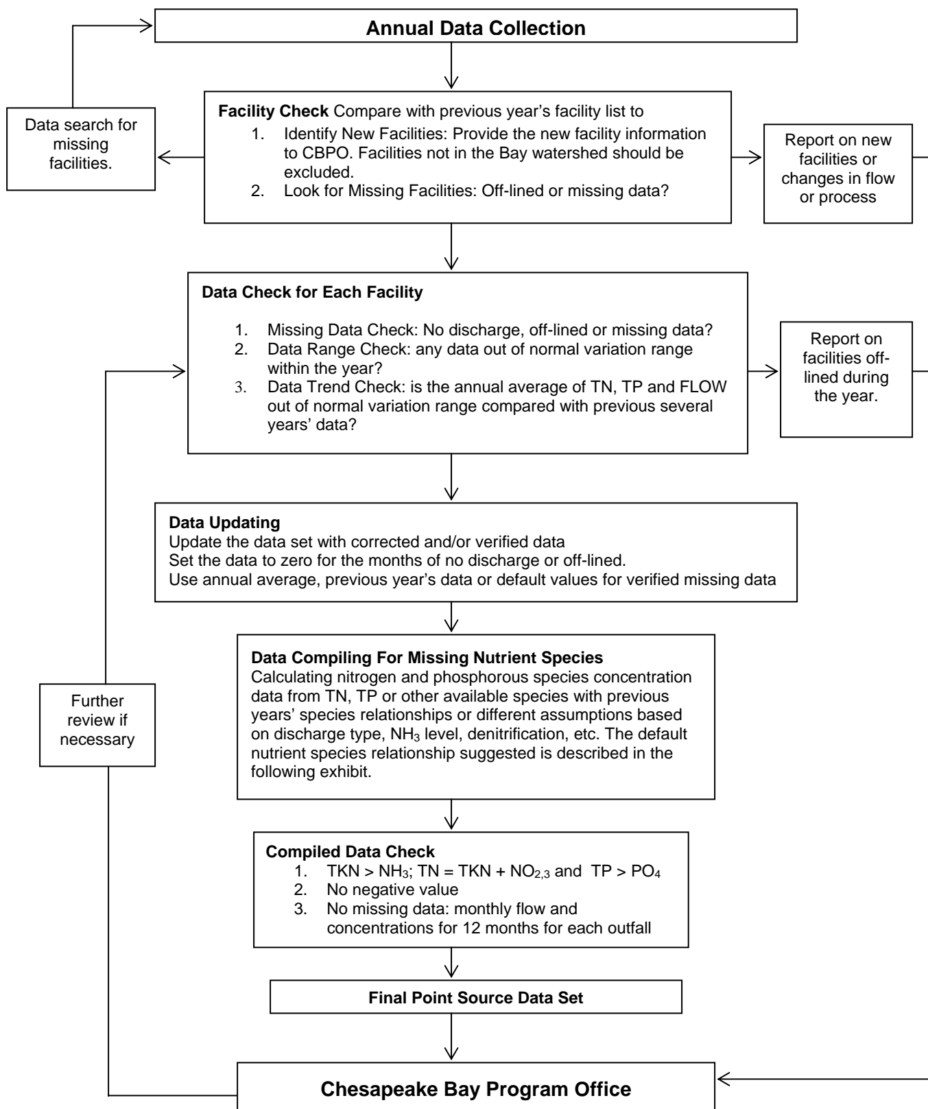
Figure 7-7 Point source nutrient data processing flow diagram.
