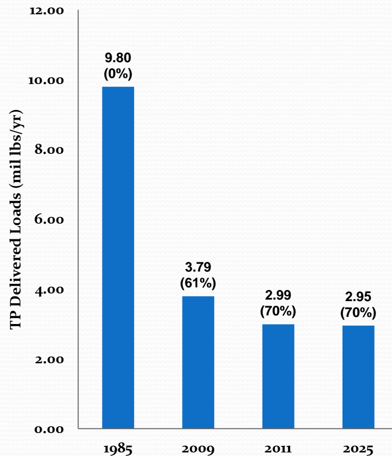
Wastewater TP Delivered Loads and Reduction (%) from 1985
