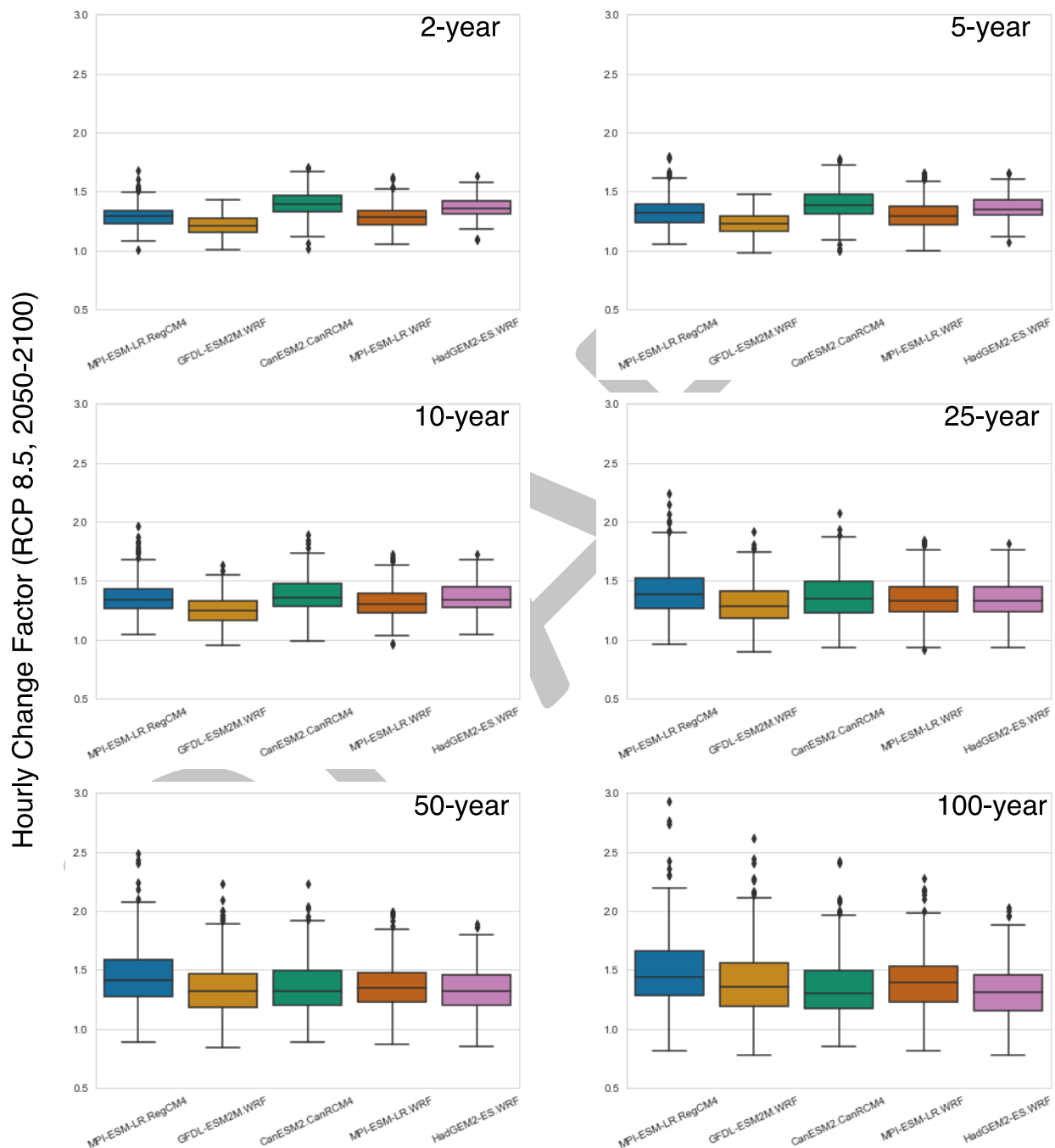
Figure 4.4. Analysis of sub-daily NA-CORDEX (50 km) change factors for RCP 8.5 (2050-2100)
