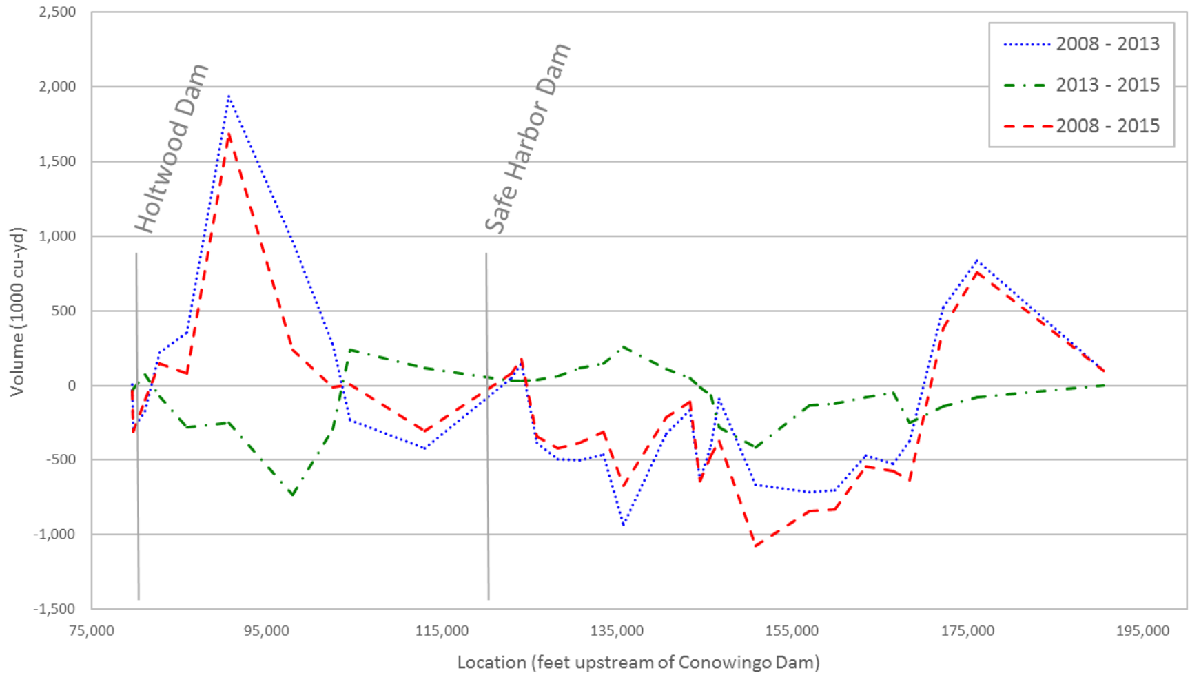
Observed Bed Volume Change in Lakes Aldred and Clarke (2008-2015)
