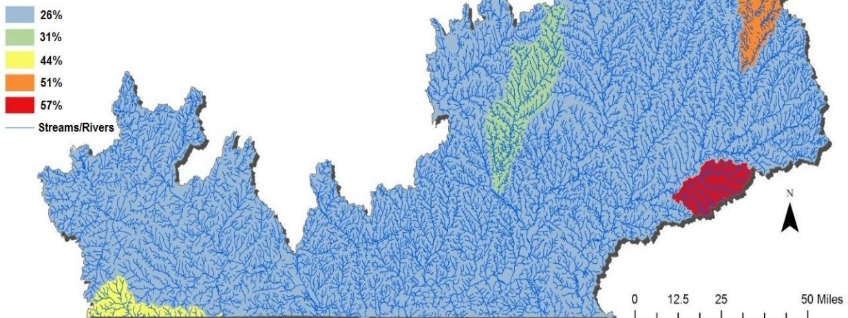
Figure 3. Percent Change in Phosphorus Delivery Factor by Land-River Segment
