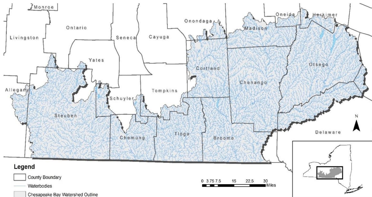
Figure 1. Chesapeake Bay Watershed boundary in New York
