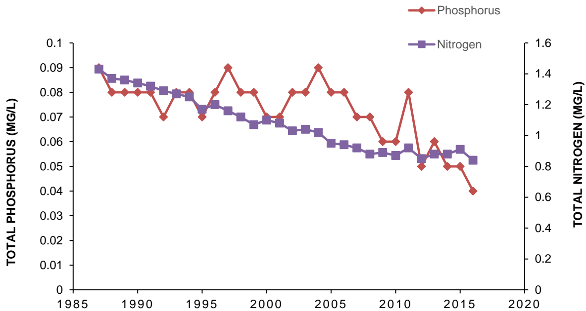
Figure 5. Long-term trend of nitrogen and phosphorus concentrations at Towanda, PA 4
