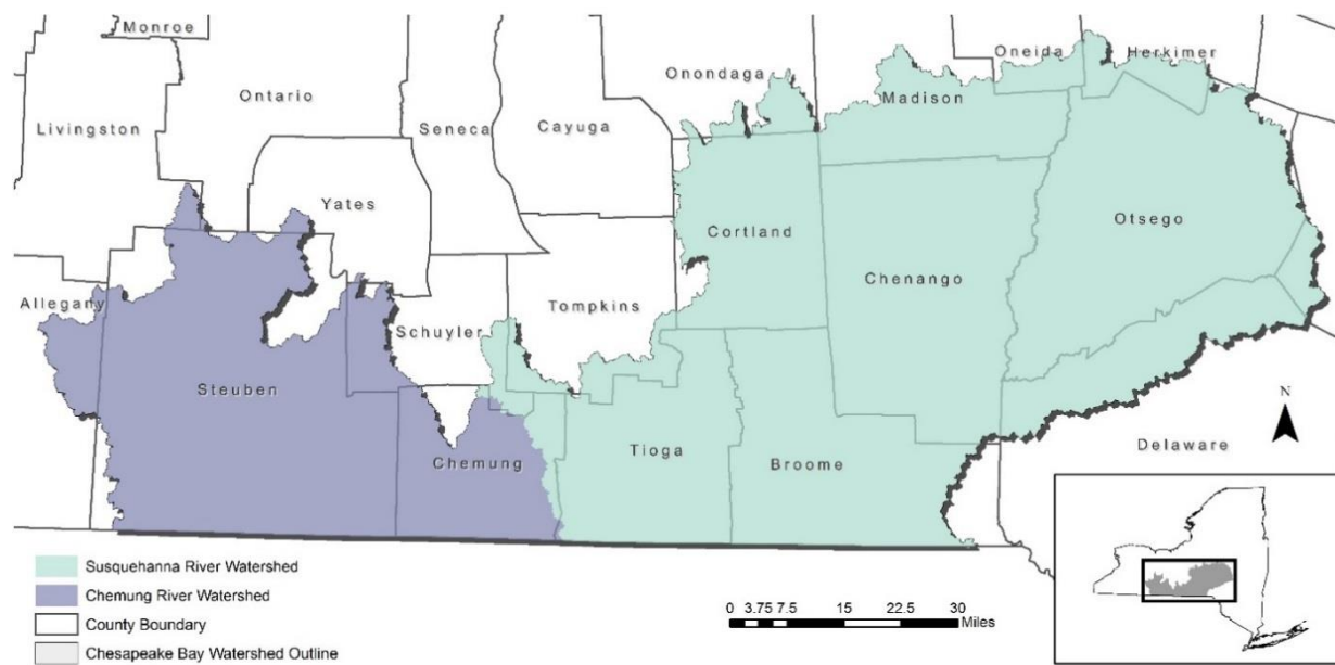
Figure 7. Agricultural Sector Local Planning Goal Watersheds
