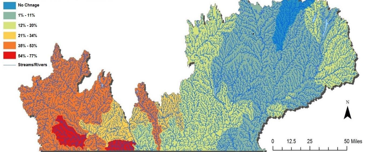
Figure 2. Percent Change in Nitrogen Delivery Factor by Land-River Segment
