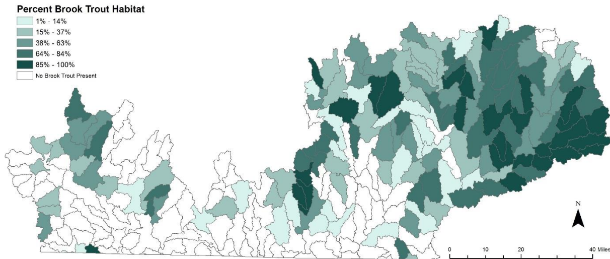
Figure 12. Percent Brook Trout Habitat in HUC 12 watersheds
