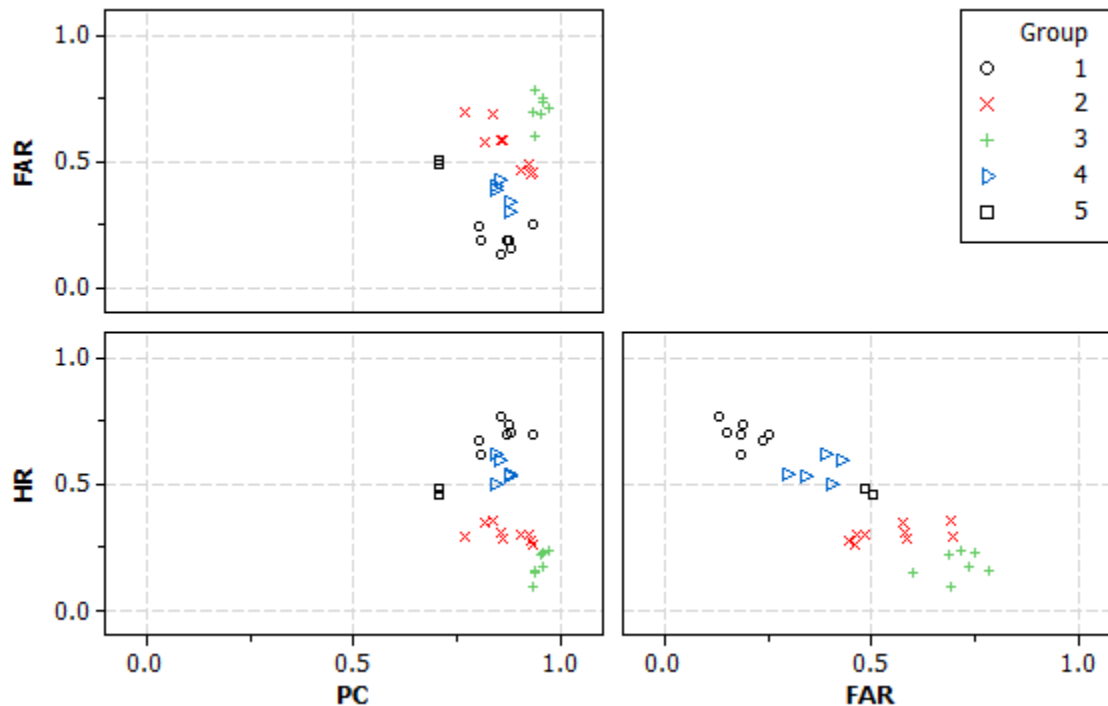
Figure 3. Cluster analysis results
