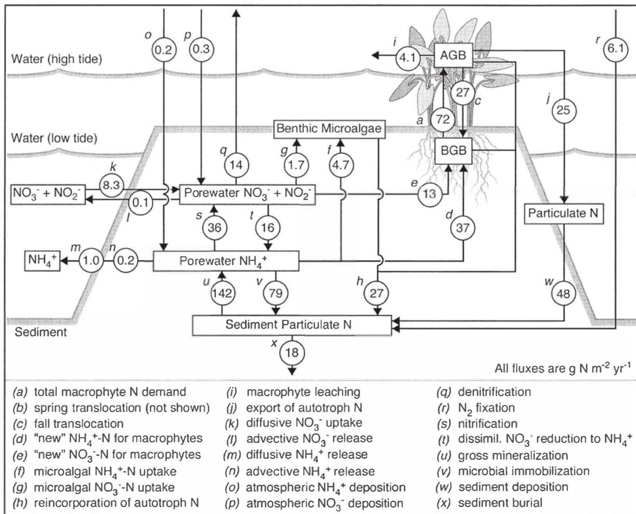
Fig. 3. Nitrogen mass balance for Sweet Hall marsh. All fluxes are in g N m -2 yr -1 and are based on measured rates, literature values, or calculated by difference (assuming steady state) as detailed in the text. Standard deviations for each flux are omitted for visual clarity but can be found in Table 1 and in the text. AGB = aboveground macrophyte biomass; BGB = belowground macrophyte biomass.
