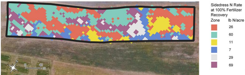
Figure 3. A variable rate prescription, accounting for differences in soil texture, soil organic matter, cover crop N content and cover crop C:N ratio.
